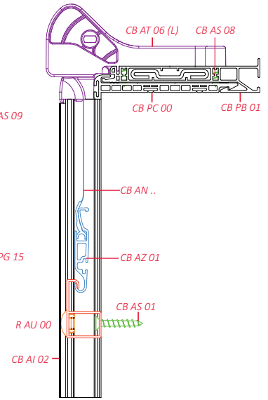
view from side B-B
