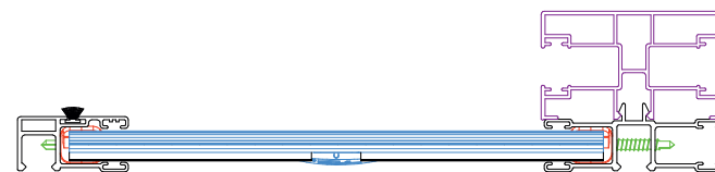
view from above (without AT, PB i PC)
