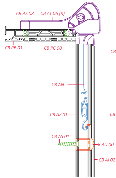
view from side A-A
