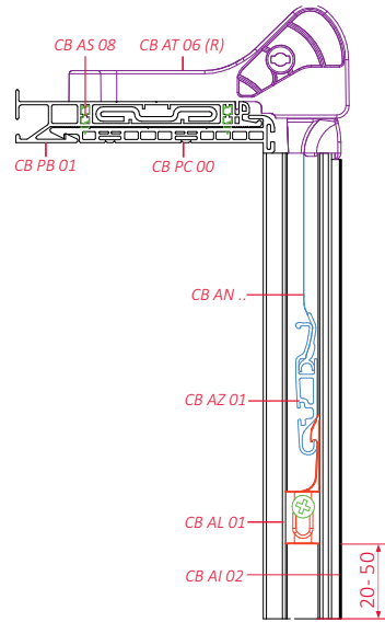
view from side A-A
