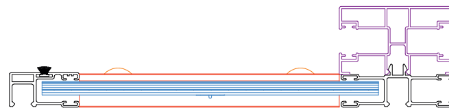
view from above (without AT, PB i PC)
