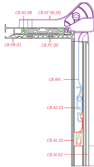
view from side A-A
